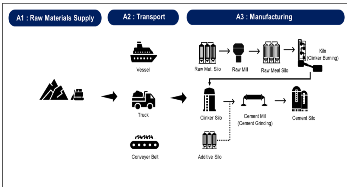
Figure 3: Information Modules of Cement production process
