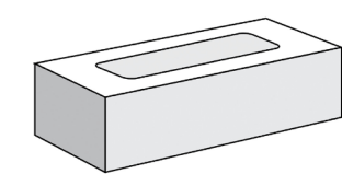
230L x 110W x 76H mm Pressed Bricks
