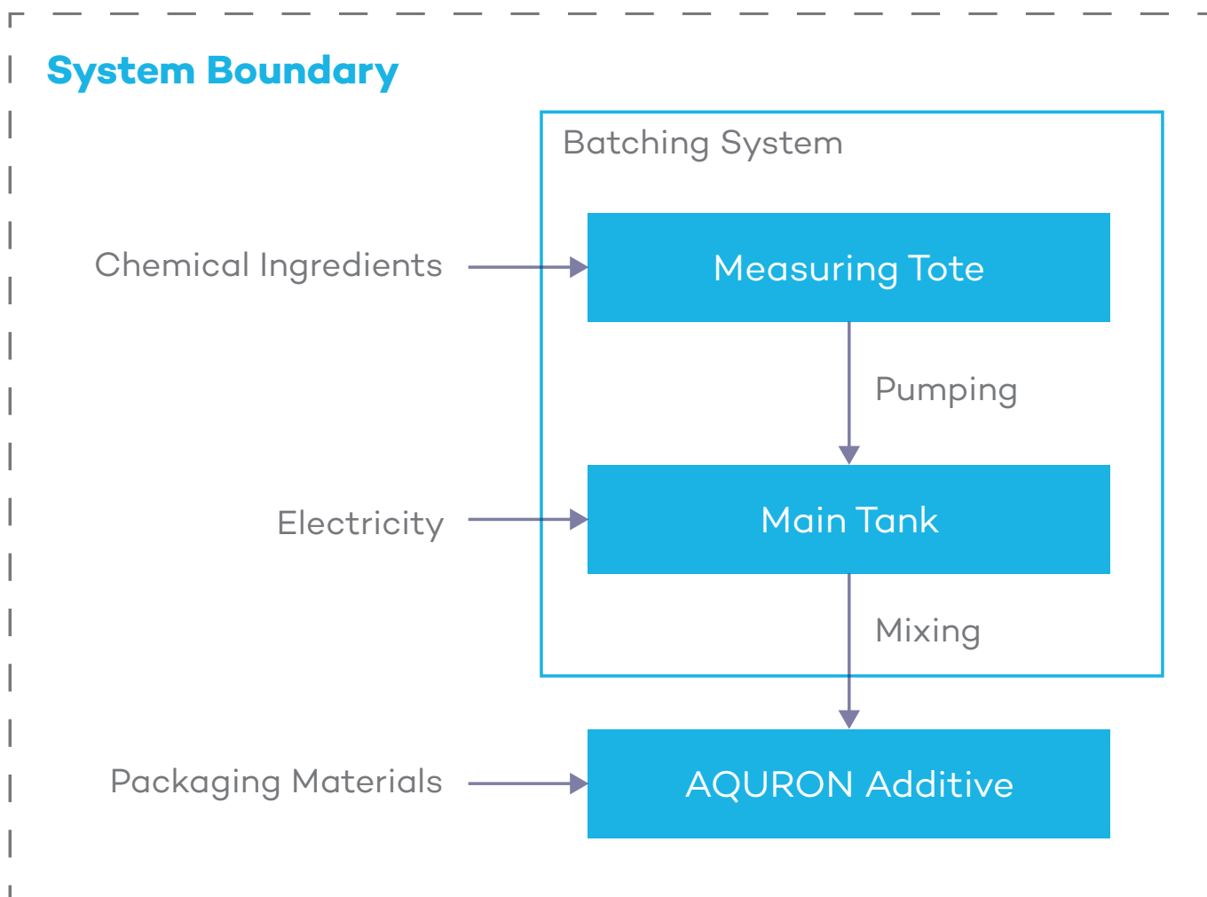
Figure 2: High level manufacturing processes (A1-A3)
