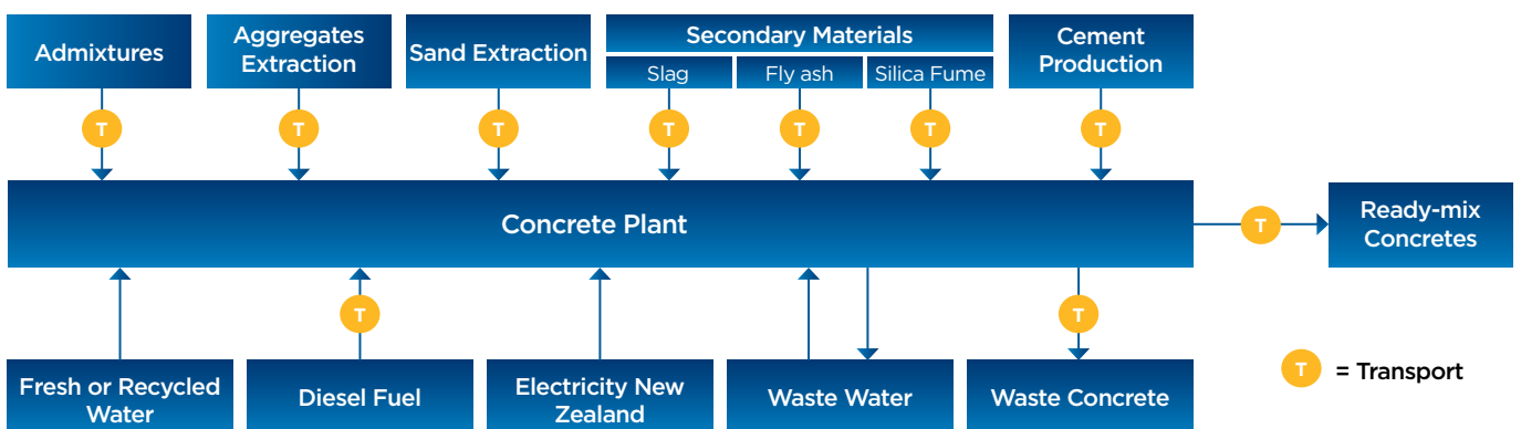
Figure 1. Manufacturing Process
