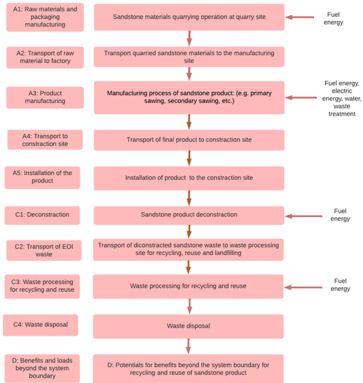
Figure 1. System diagram
