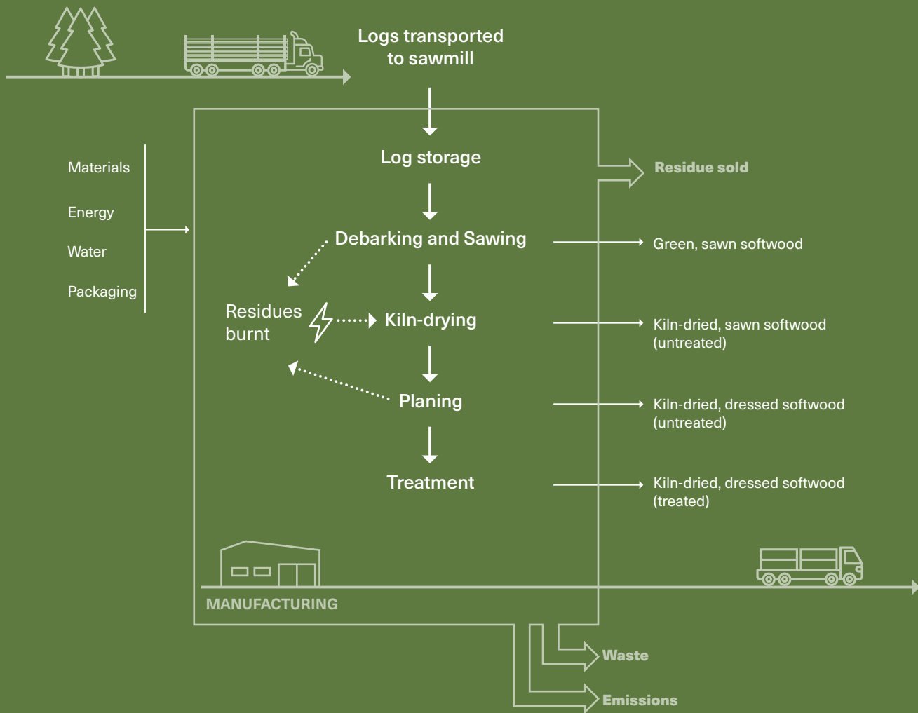
Figure 1: Manufacturing (A1-A3) process flowchart .
