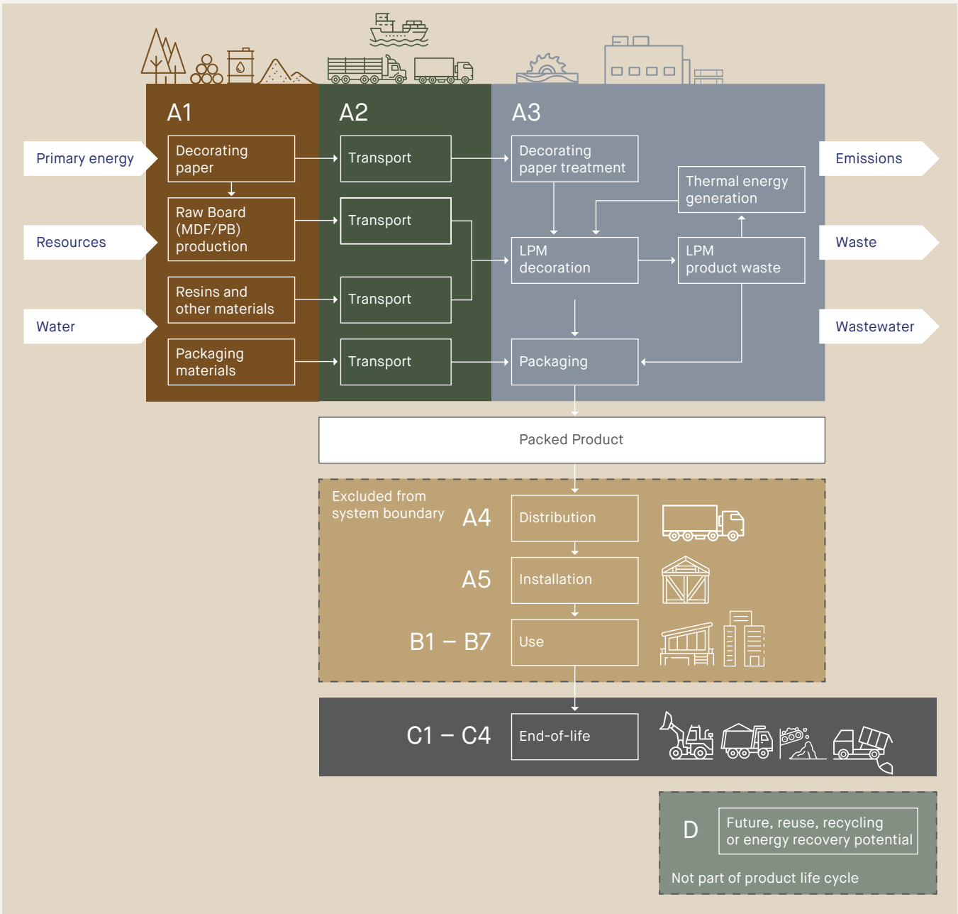
Figure 2: Laminex® Architectural Wall Panels (Classic Flat) system boundary diagram
