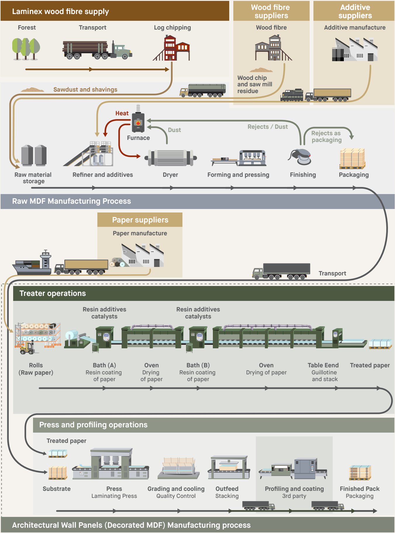
Figure 1: Laminex® Architectural Wall Panels manufacturing process
