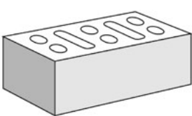
230L x 110W x 76H mm 8 Hole Bricks
