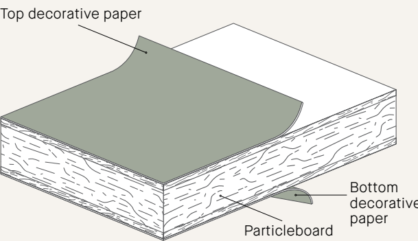
Figure 1: Decorated Particleboard
