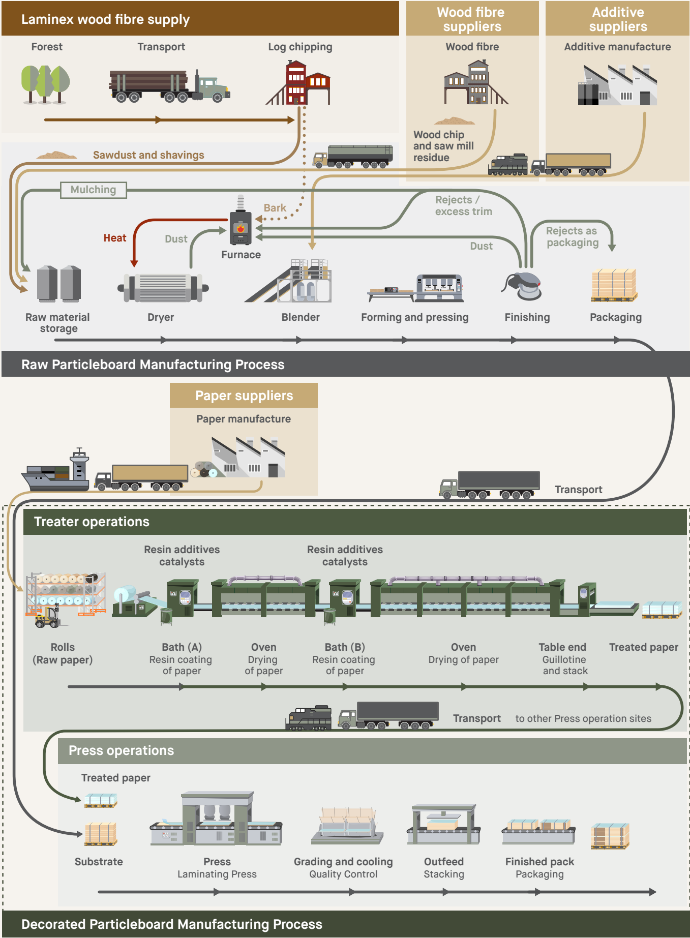
Figure 2: Decorated Particleboard manufacturing process
