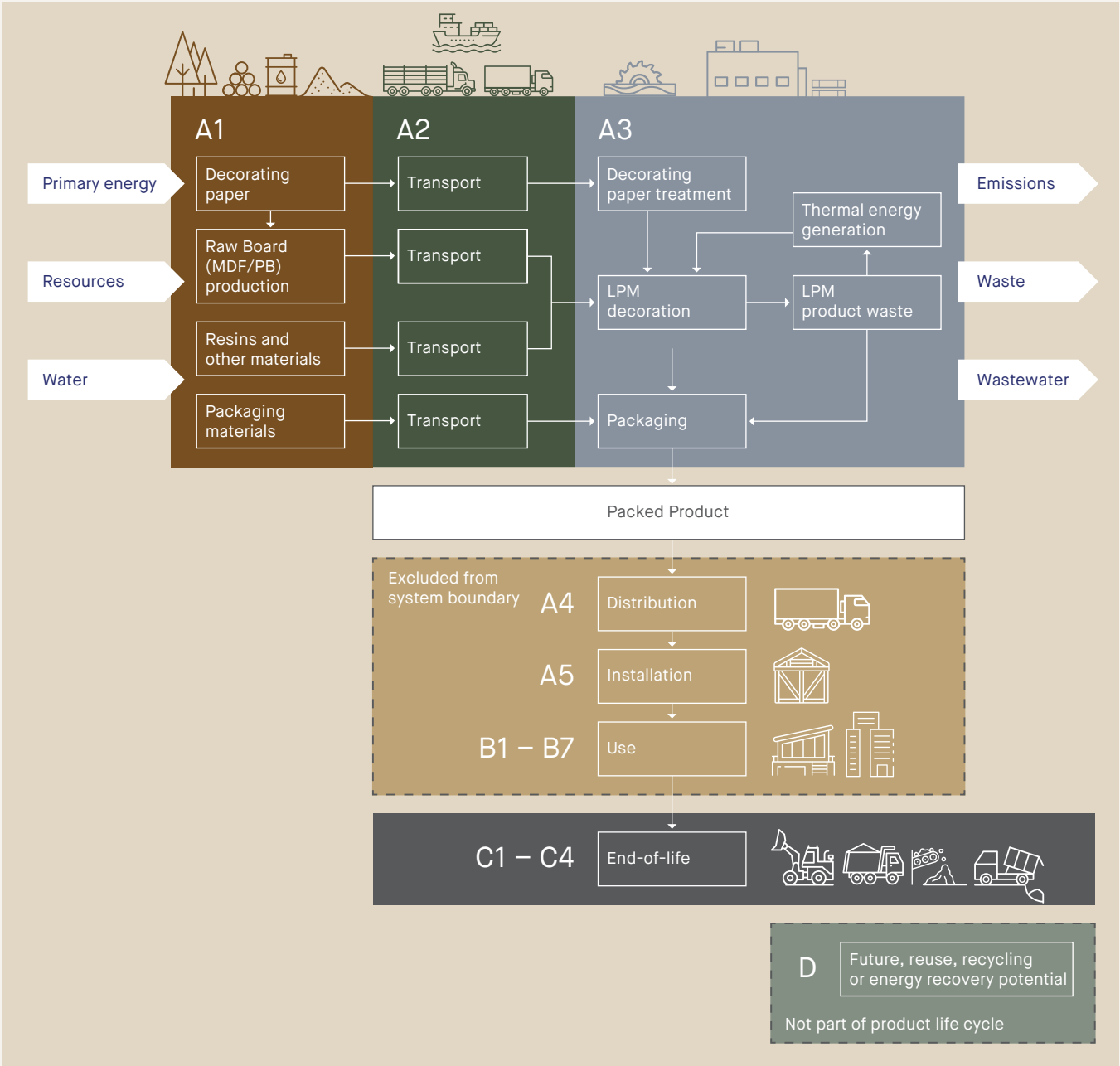
Figure 2: Laminex® Architectural Wall Panels (Profiled) system boundary diagram
