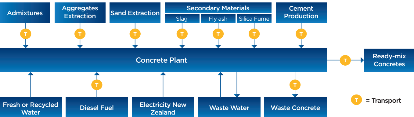
Figure 1. Manufacturing Process
