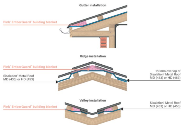
Diagram 3: Typical Residential roofing Pink EmberGuard Building Blanket installation
