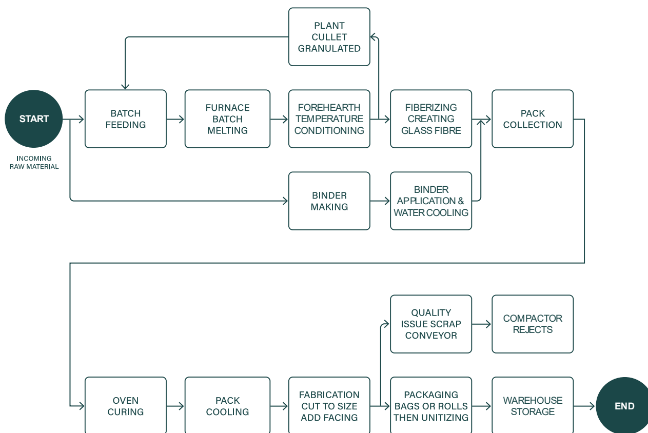
Diagram 3: Glasswool manufacturing process flow
