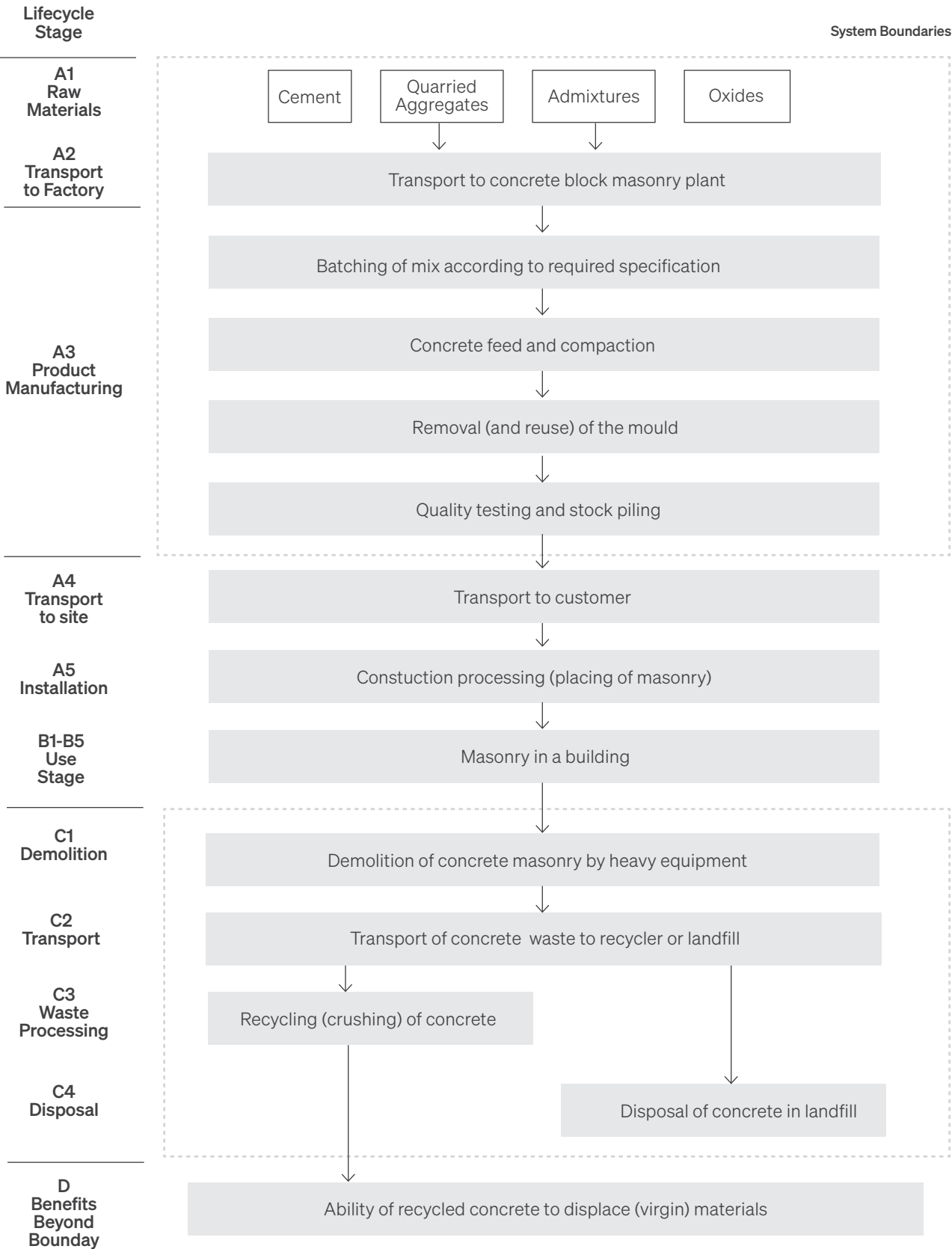
Figure 2: Life cycle stages of Austral Masonry concrete
