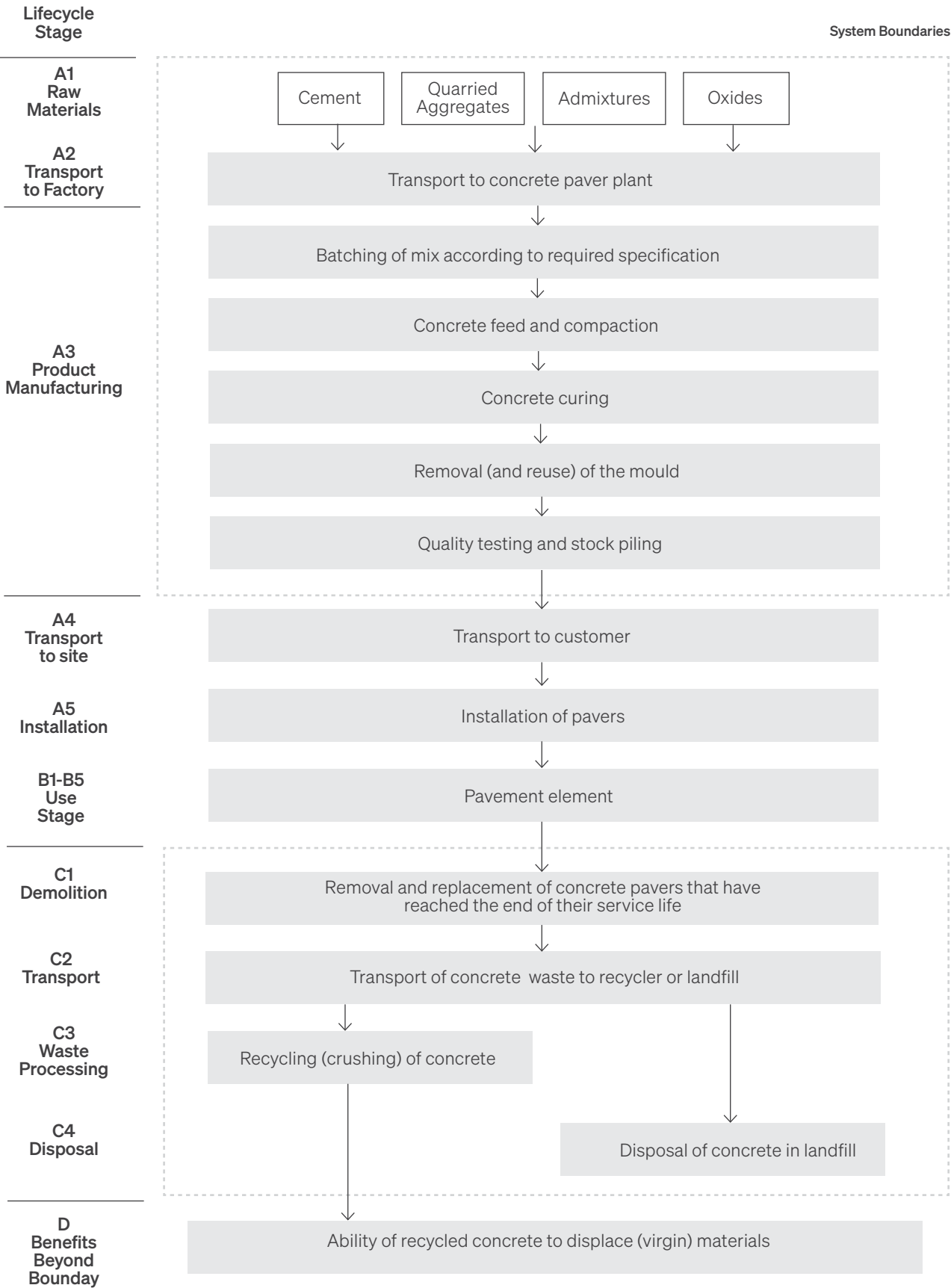
Figure 3: Life cycle stages of Austral Masonry dark concrete pavers
