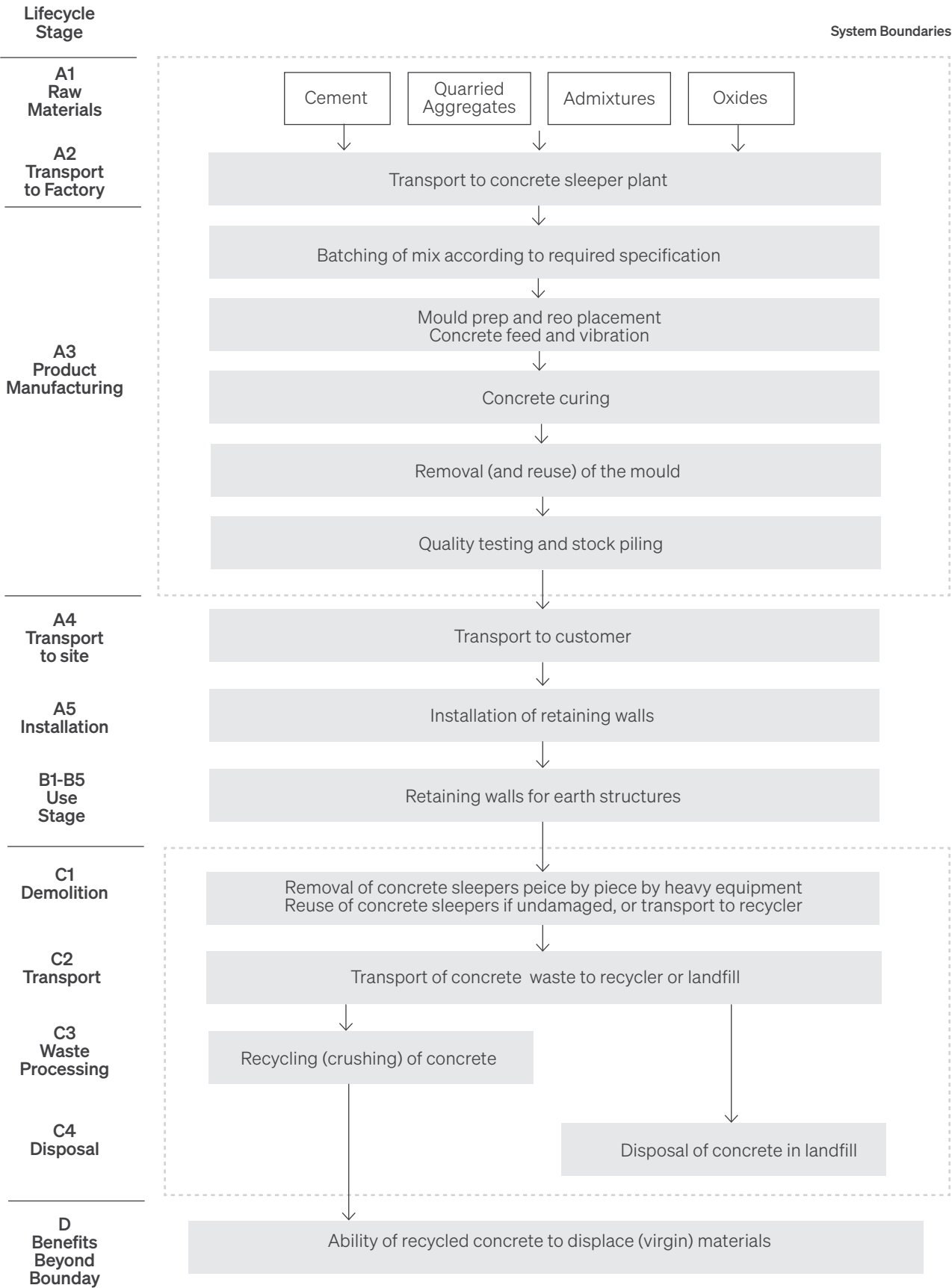
Figure 3: Flow diagram of the life cycle of retaining wall products
