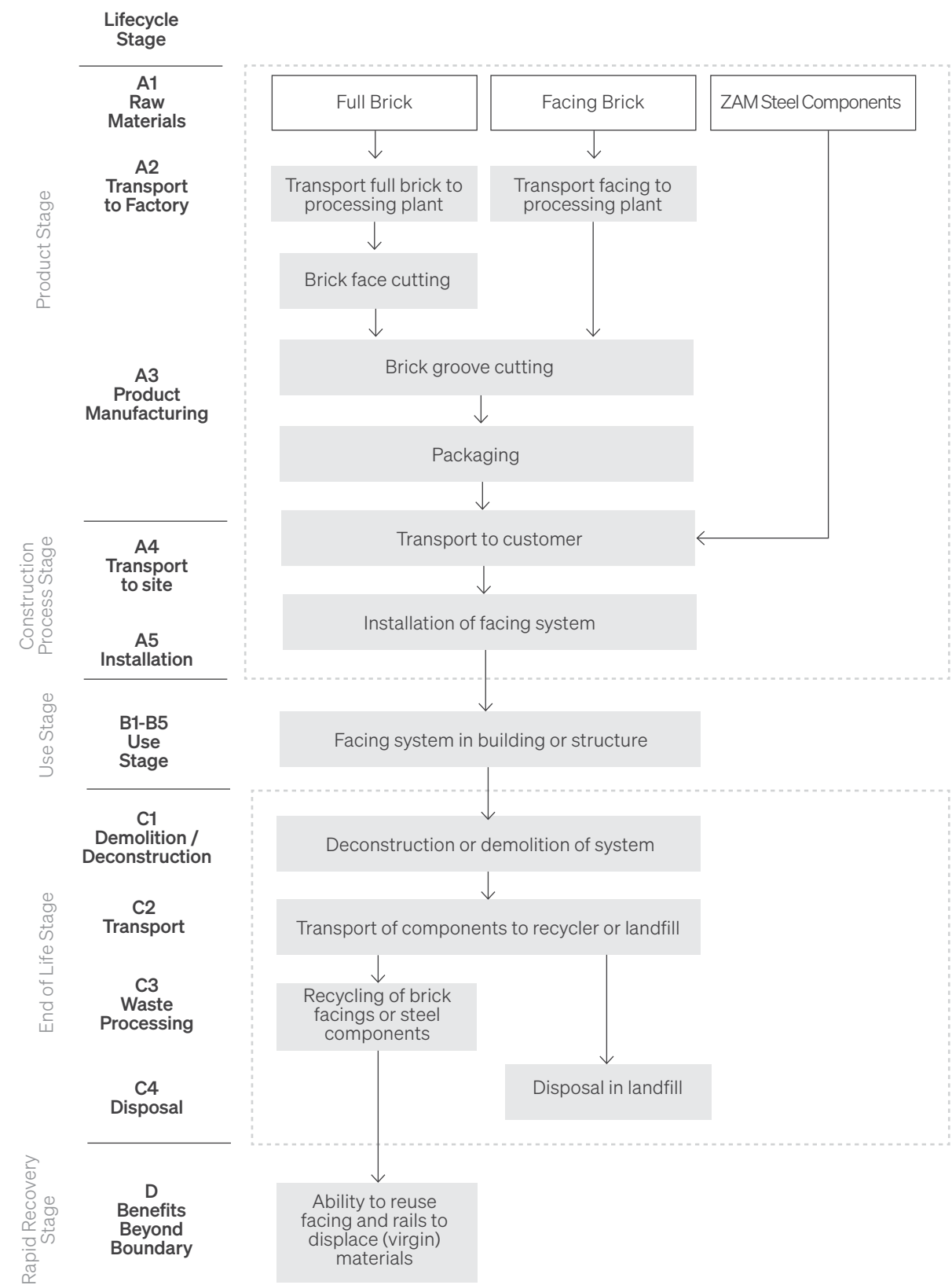
Flow Diagram of the Life Cycle of Thin Tech Plus
